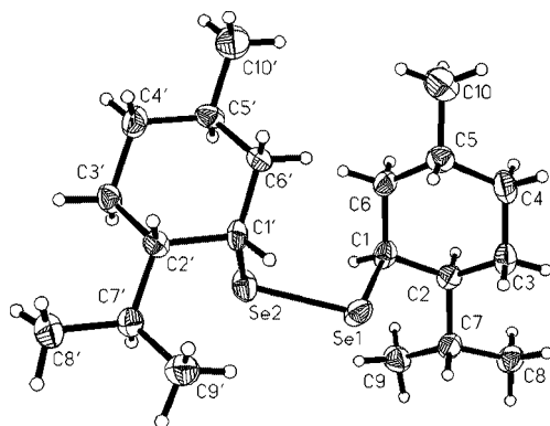
Figure 1. X-ray structure of (+)-dineomenthyl diselenide ( 4 ). Selected bond lengths [Å] and angles [°]: Se(1)–Se(2) 2.3182(11), Se(1)–C(1) 2.008(8), Se(2)–C(1') 1.990(7); C(1)–Se(1)–Se(2) 100.6(2) C(1')–Se(2)–Se(1) 100.05(18).
